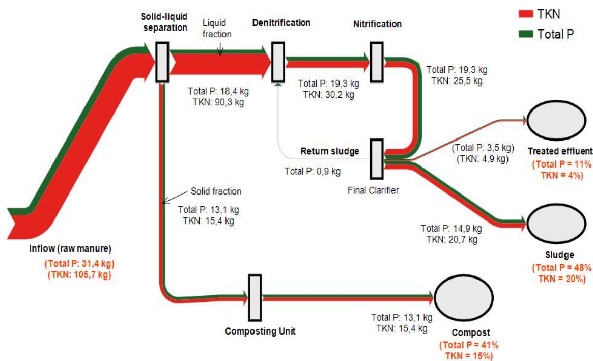
Figure 3.11 Illustration of TKN and P flows (in kg.day) from an NDN plant in Caldetenes, Spain (adapted from Foged et al. , 2011a).
