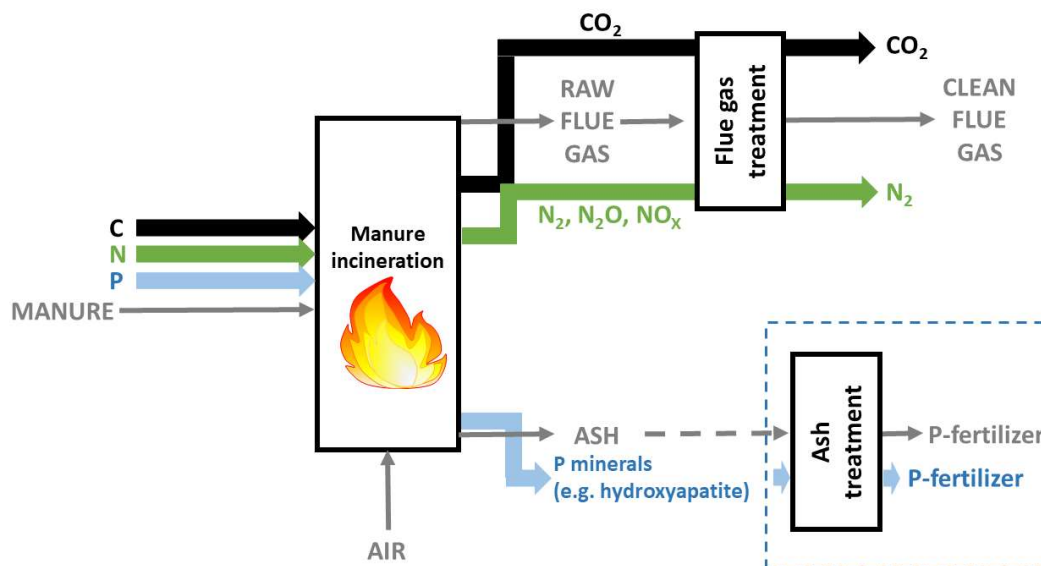
Figure 3.9 Simple schematic mass and elemental flow during manure incineration.
