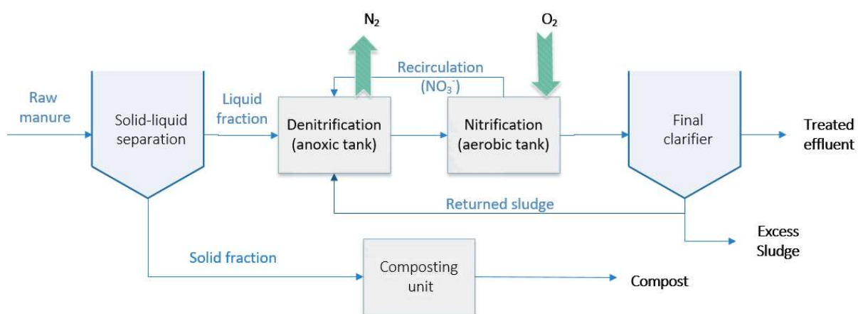
Figure 3.10 Process flow of a Nitrification-Denitrification system for N removal
