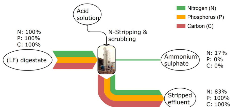
Figure 3.14 N, P and C fate during digestate processing by means of N-stripping, where 17% of total N is recuperated as ammonium sulphate solution. Adapted from Bolzonella et al. (2018).
