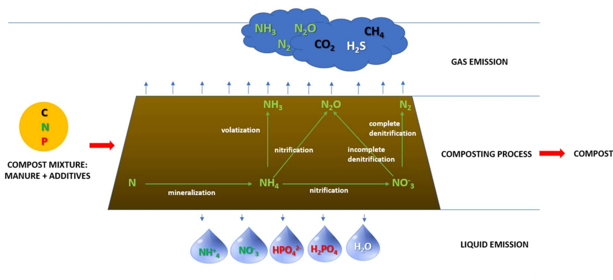
Figure 3.8 The flow of C, N, P during composting.
