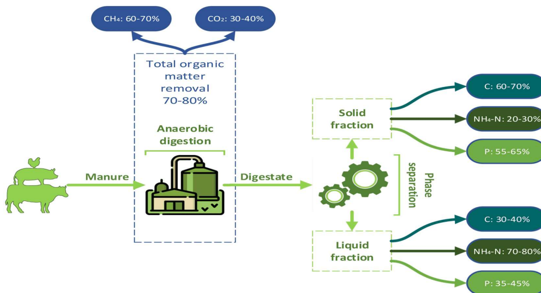
Figure 3.4 Schematic representation of CNP flows from digested manure
