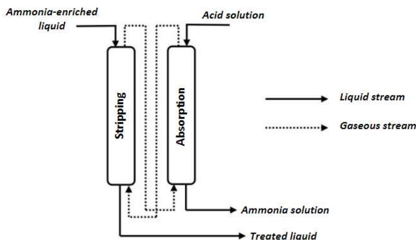
Figure 3.13 Schematic overview of the N-stripping process (Bernal et al. , 2015).
