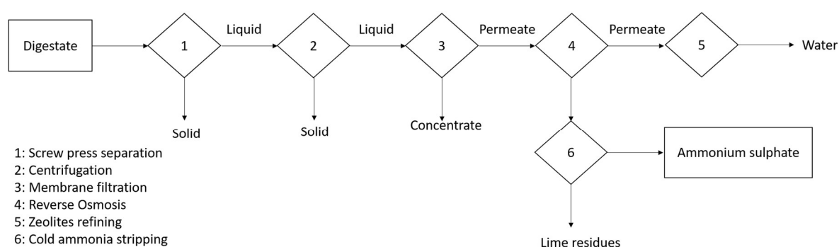
Figure 3.7 Six-step approach of the membrane plant (after Fangueiro et al., 2017)
