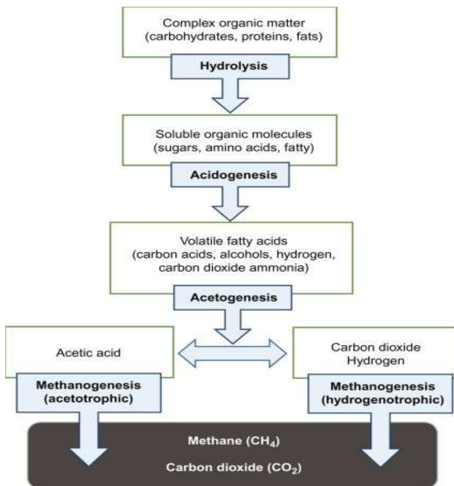
Figure 3.2 Main steps of the anaerobic digestion process (Fardin et al. , 2018)
